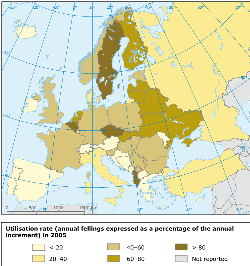
Map 3.1 Intensity of forestry – net harvesting rate in 2005
