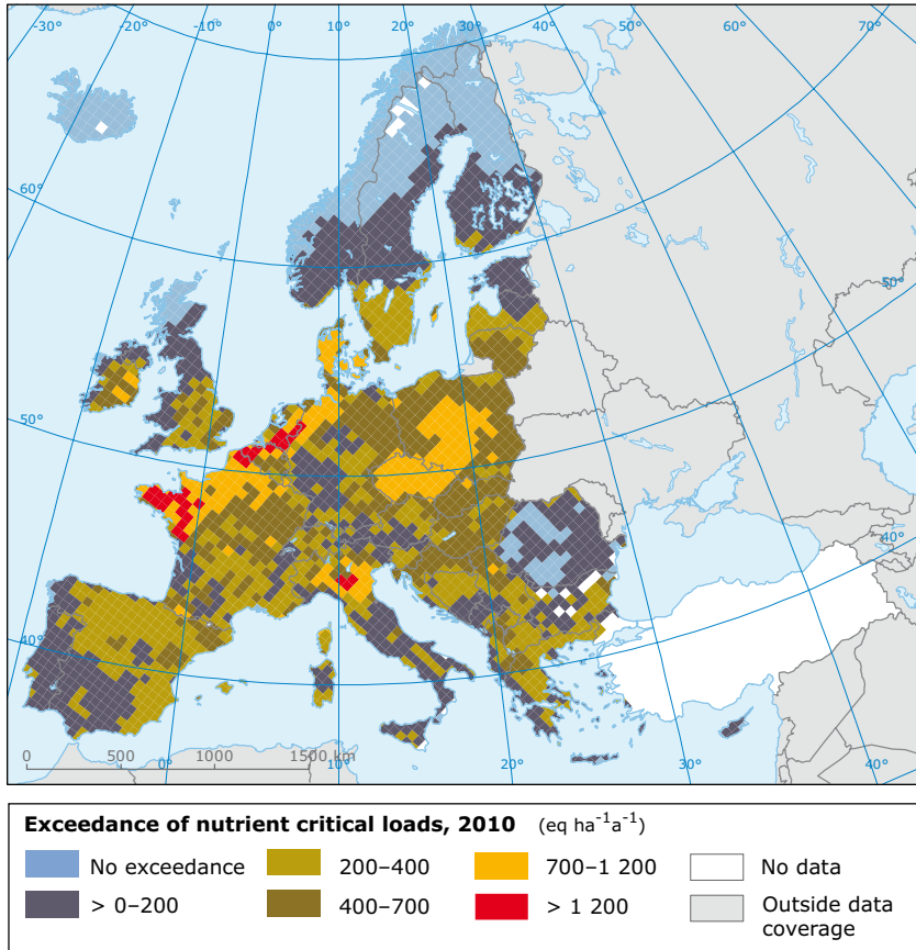
Map 3.4 Exceedances of critical loads for eutrophication due to the deposition of nutrient nitrogen in 2010
