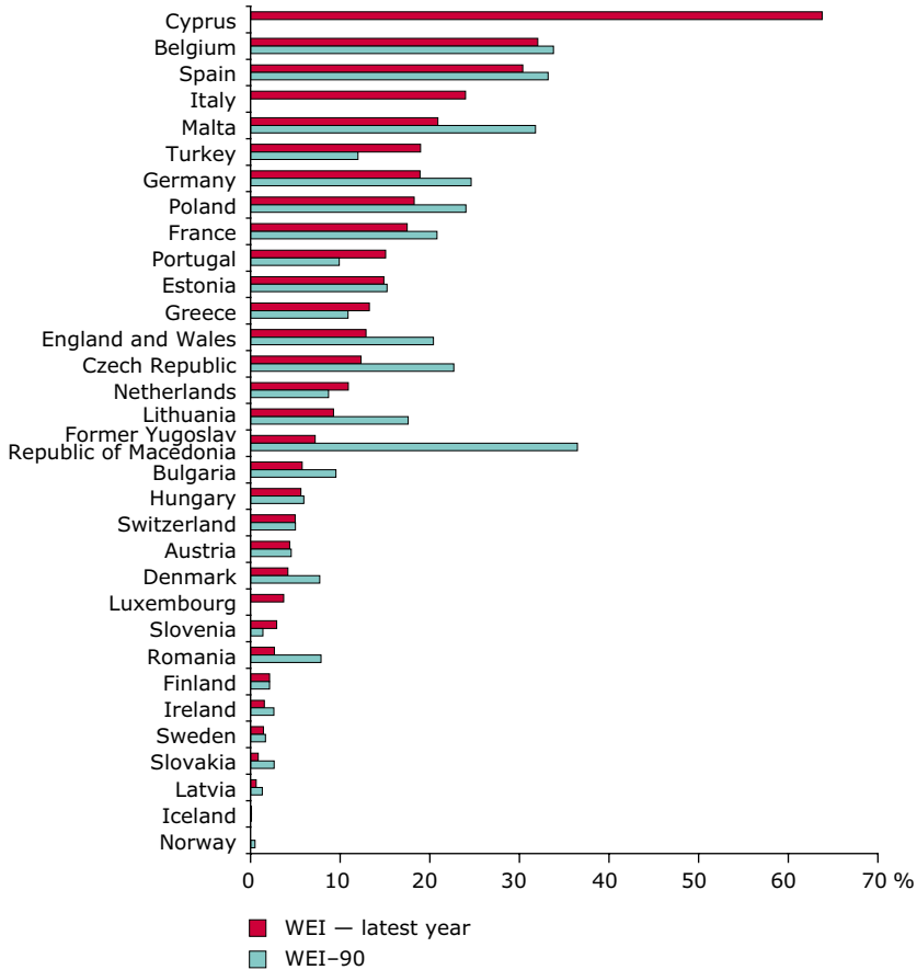
Figure 4.6 Water exploitation index (WEI) – in late 1980s/early 1990s (WEI-90) compared to latest years available (1998 to 2007) (F)
